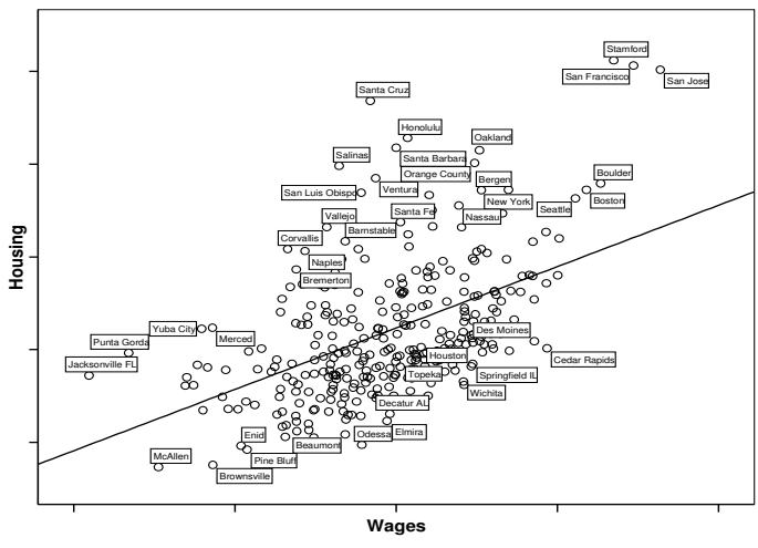
Fig 3: Scatter-graphs
