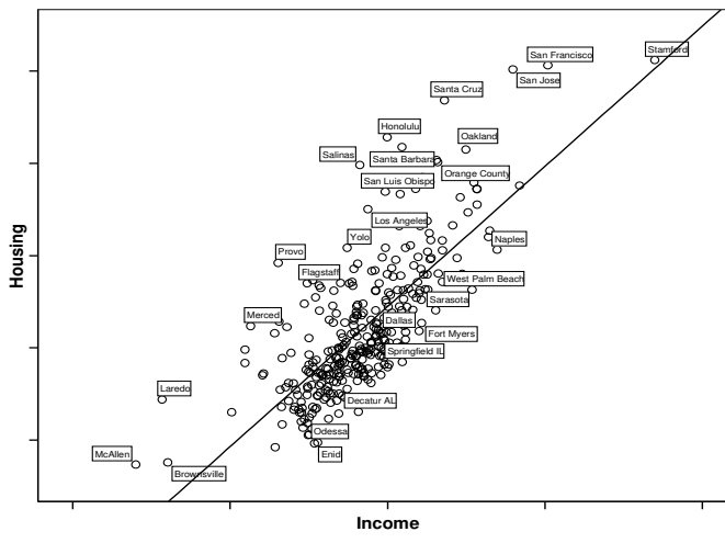
Fig 3: Scatter-graphs
